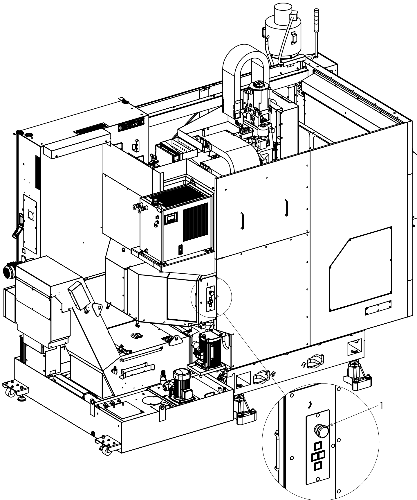
Tool Loading Station Panel
